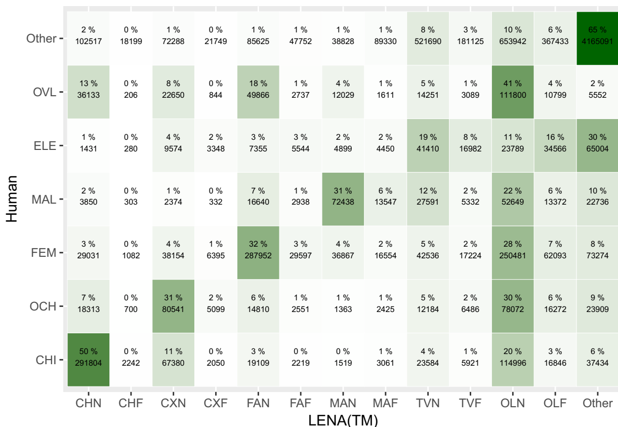
Fig. 3 Recall: Confusion matrix between LENA (x-axis) and human annotations (y-axis). In each cell, the top number indicates the percentage of all frames that a human labeled as a given class (row) which
